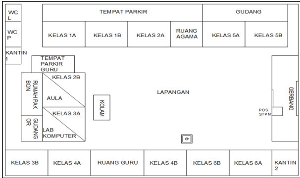
Gambar 3. Site Plan SDN Joglo No 76
